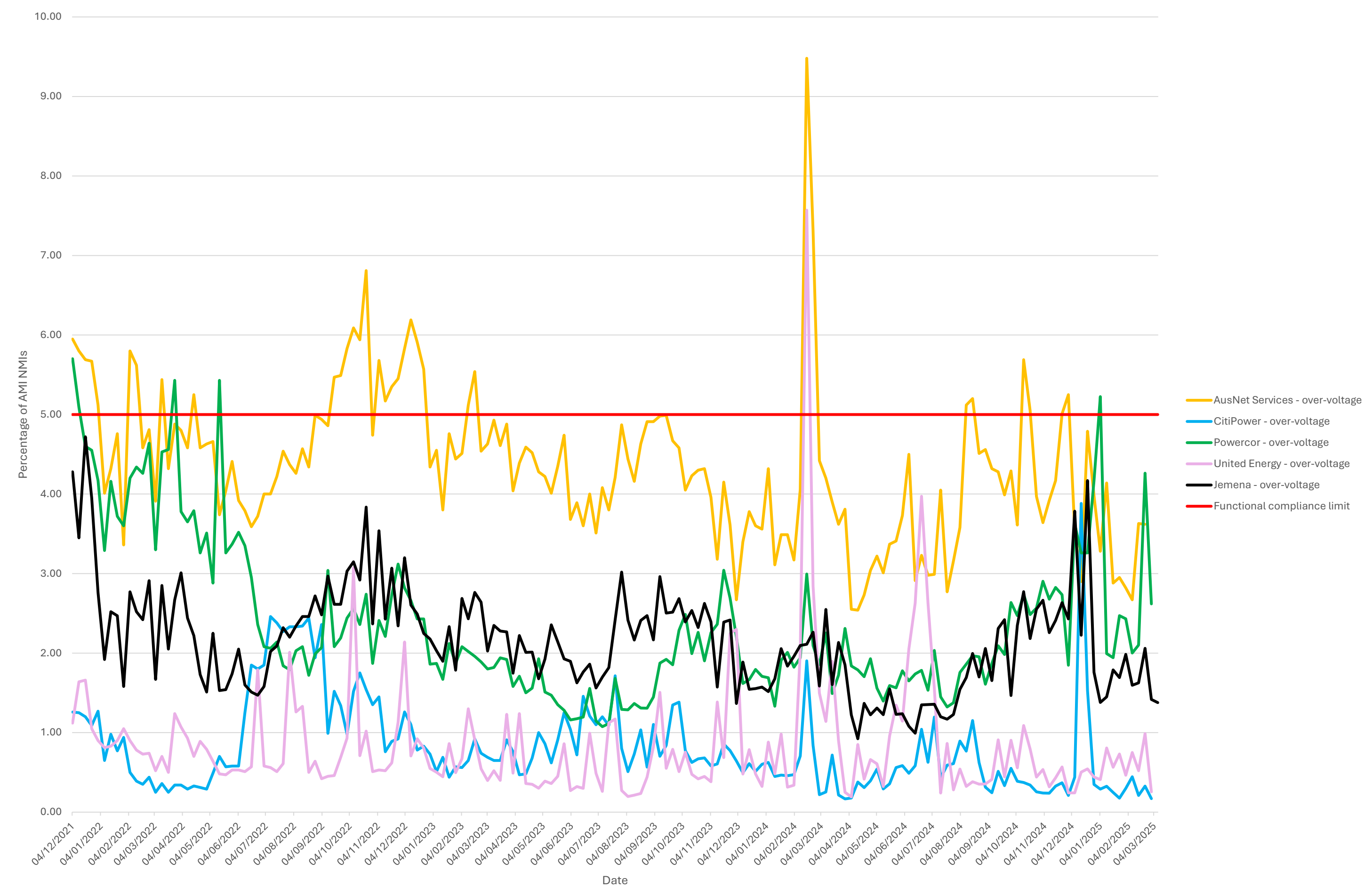
Graph 1: % of NMIs above 253V for more than 1% of the time (over-voltage)
