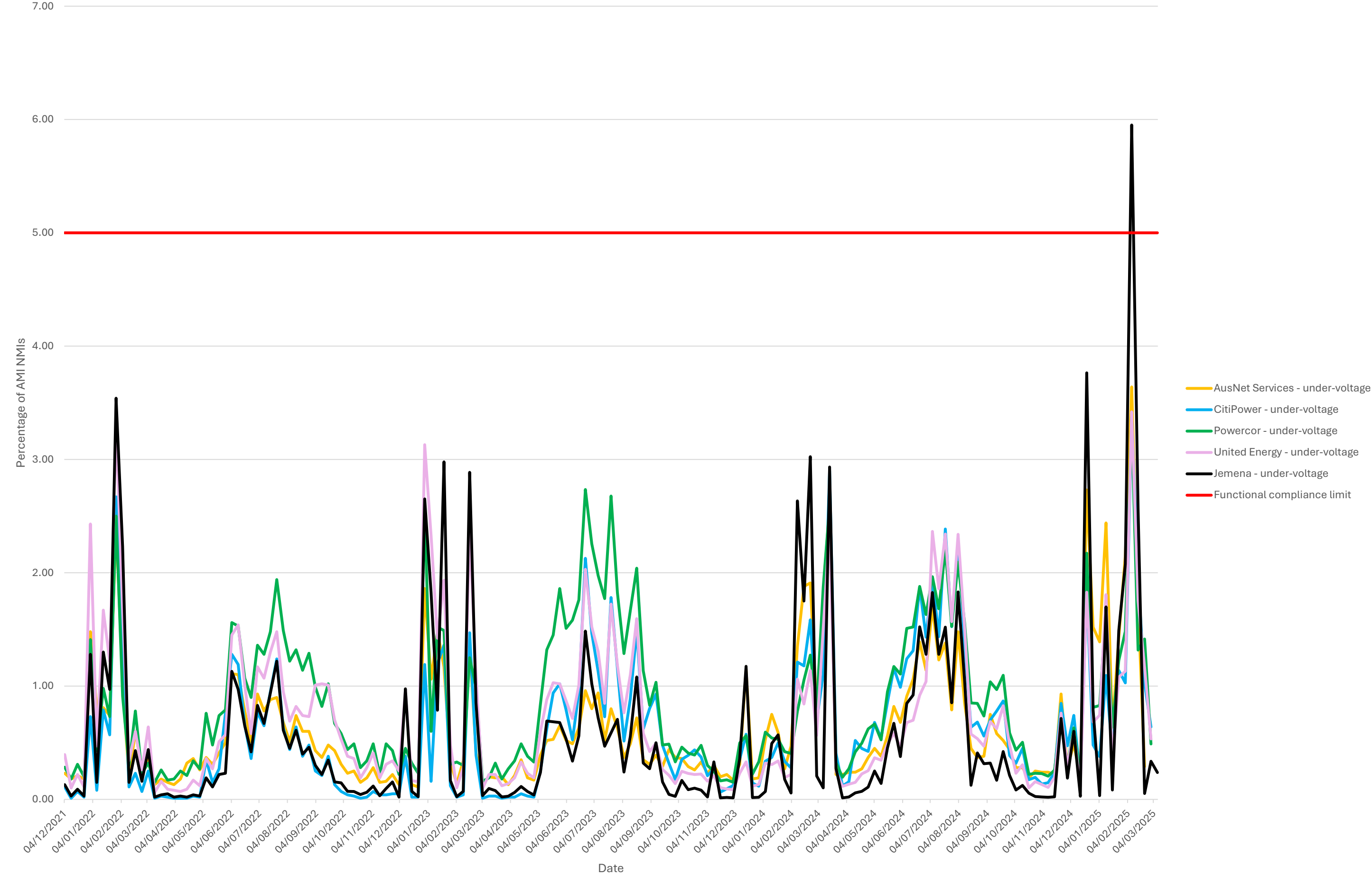
Graph 2: % of NMIs below 216V for more than 1% of the time (under-voltage)
